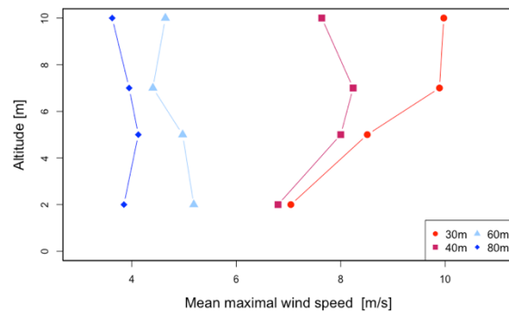
Figure 5 :: Vertical profile of the mean maximum wind speed
