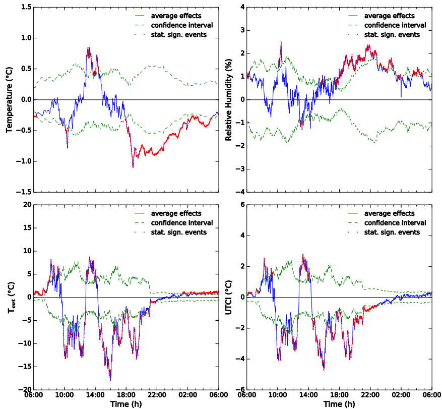
Figure 16: Microclimatic impacts of the site's renovation. Assessment based on 18 observation days before and 18 after conversion. Results are given in local time (UTC+2).
