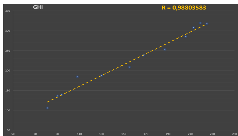
Figure 3. Correlation between experimental and software-simulated mean monthly GHI ( W/m^2 ) data for the year 2020.
